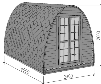
Assembled sauna pod
