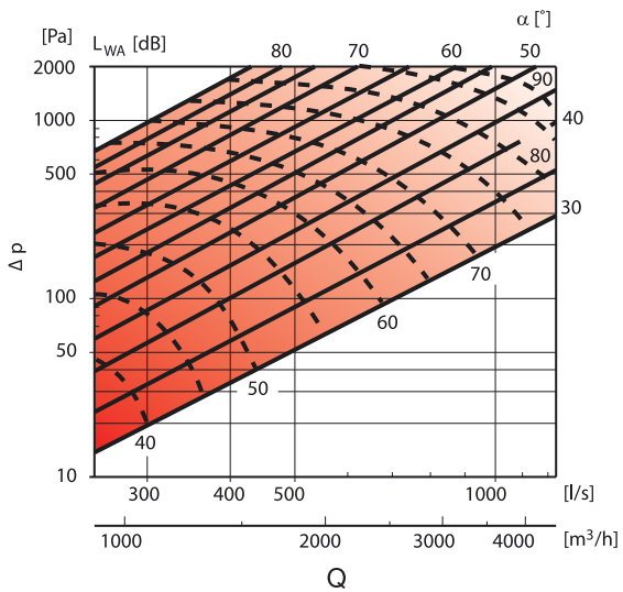
AKH Ø315
