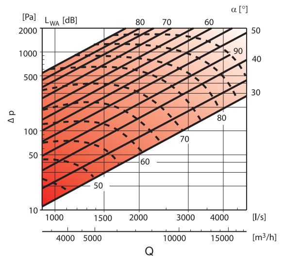
AKH Ø630
